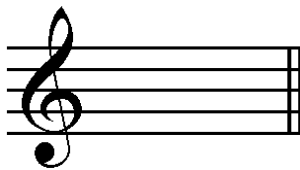
g minor
